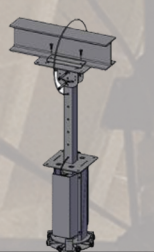
Extension Kit & Angle Bracket
